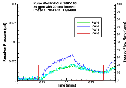
Hydraulic Pulse Interference Test Results
